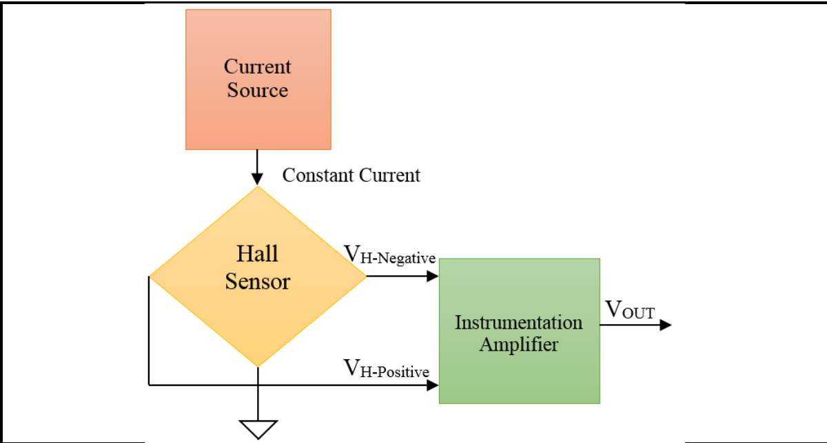
Figure 3. Recommended circuit.
